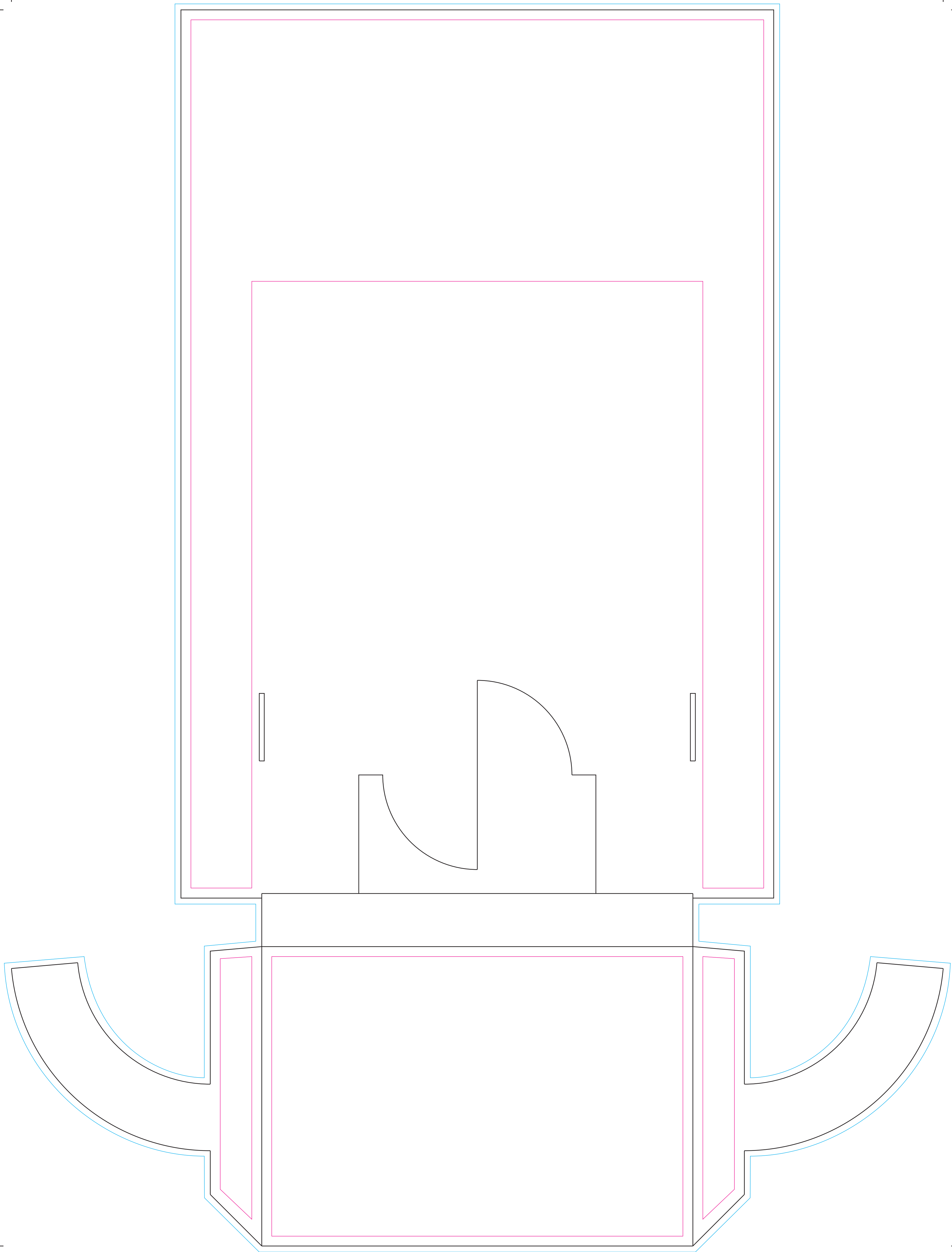
A4 Leaflet Dispenser Overall Dimension: 467mm x 619mm — Finished Size — Bleed Area — Text Limit/Quiet Border (text and photos not running to bleed should be within this area)
