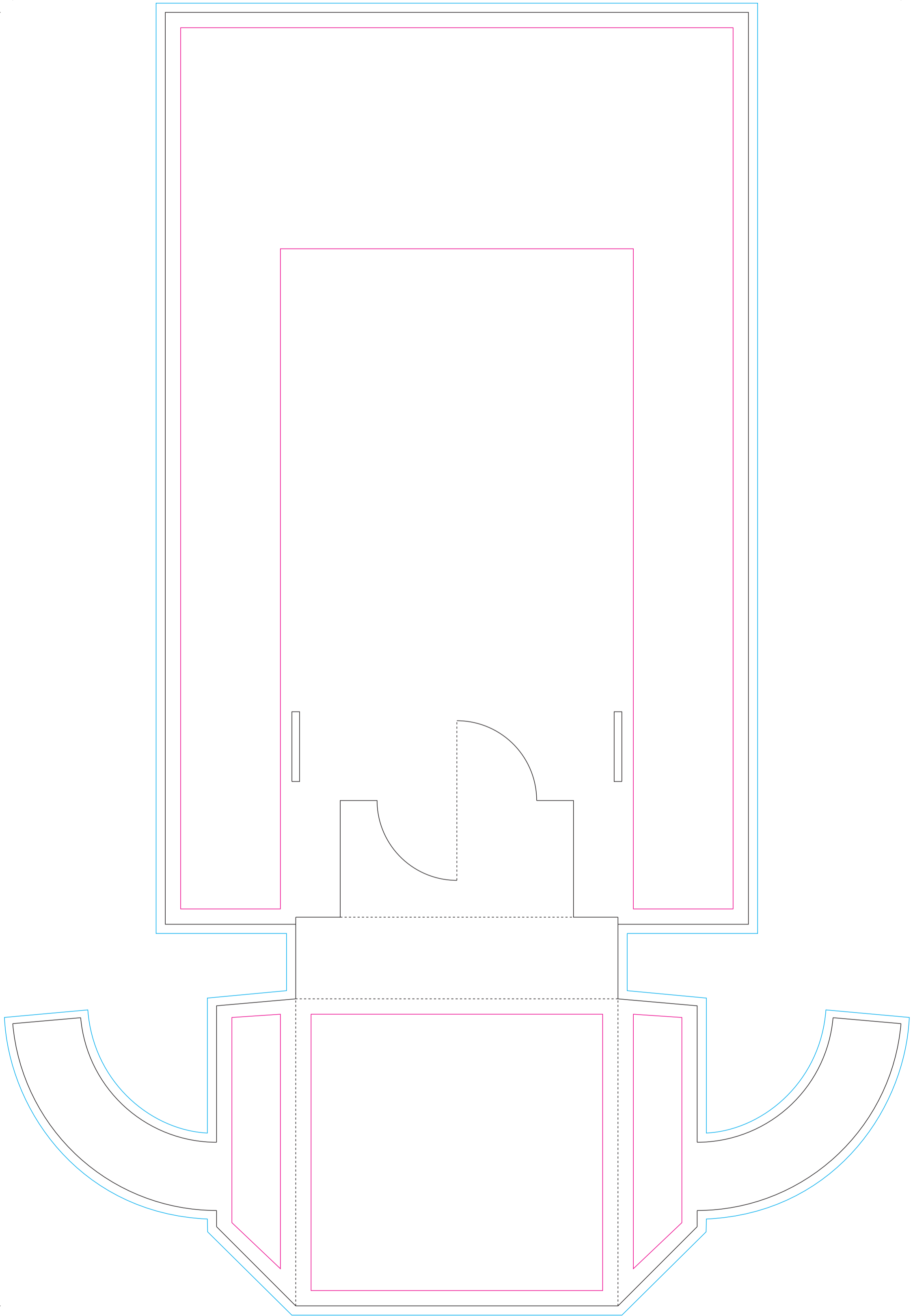
1/3 A4 Leaflet Dispenser Overall Dimension: 290mm x 421mm — Finished Size — Bleed Area — Text Limit/Quiet Border (text and photos not running to bleed should be within this area)
